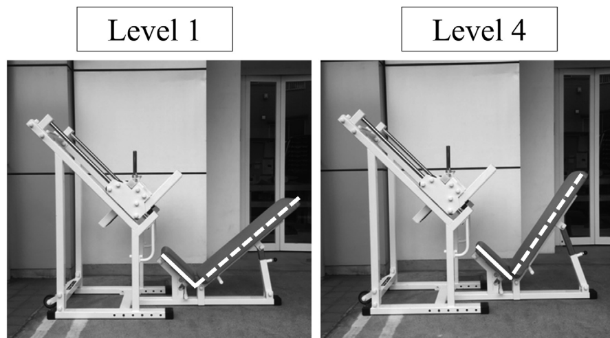
Figure 3 : Seat angle of the machine. The seat angle can be adjusted to four positions according to the flexibility of the hamstrings. The angle at position 4 is less than 90^\circ . Simply sitting on the bench produces deep hip joint flexion, which stretches the hamstrings.
