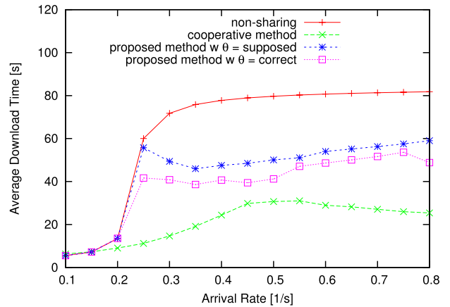
Fig. 12 Average download time ( \theta = -80 ).
