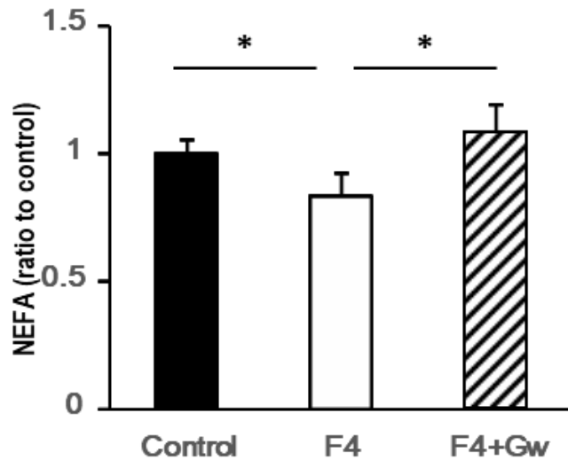
Figure 5: PPAR \alpha and its downstream targets mediate the TG and NEFA reducing effect caused by M-F4.
