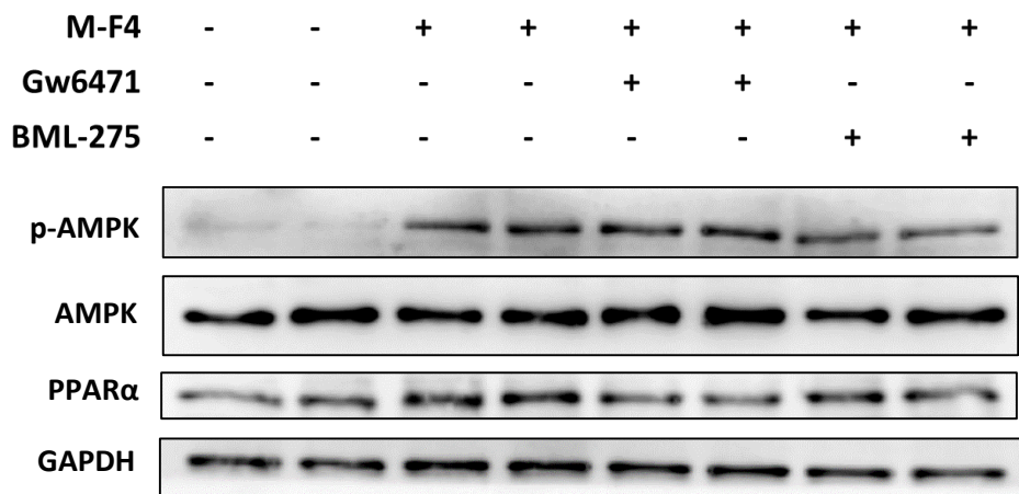
Figure 6: PPAR \alpha was the downstream target of AMPK signal pathway. C2C12 myotubes were stimulated by M-F4 (100 \mu g/mL) and treated with or without 25 \mu M Gw6471 and 15 \mu M BML-275. The proteins were examined by western blotting analysis to check PPAR \alpha and phosphorylation and total levels of AMPK.
