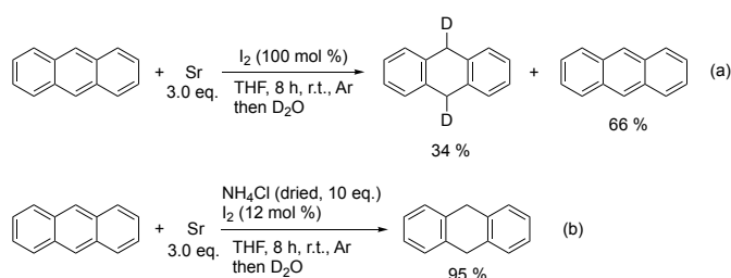
Scheme 1. Investigation of deuterium incorporation in the reduction of anthracene with strontium metal and iodine (a) or iodine/ammonium salt (b) conditions.
