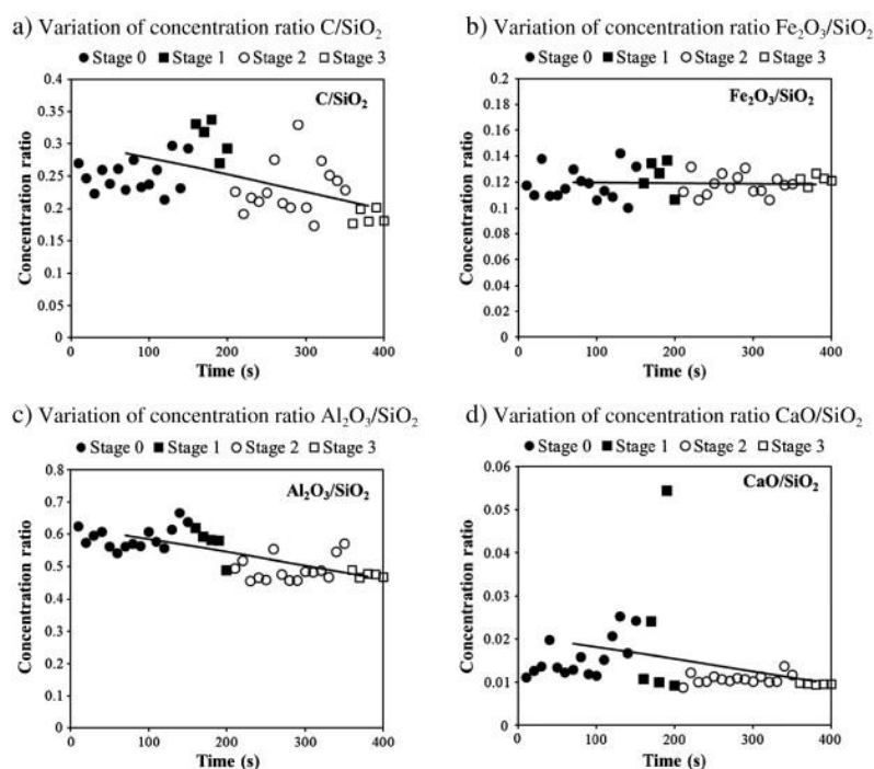
Fig. 5 Real-time LIBS measurement results of fly ash in different stages [102] (Z. Z. Wang, Y. Deguchi, M. Kuwahara, T. Taira, X. B. Zhang, J. J. Yan, J. P. Liu, H. Watanabe and R. Kurose, Quantitative elemental detection of size-segregated particles using laser-induced breakdown spectroscopy. Spectrochimica Acta Part B: Atomic Spectroscopy , 2013, 87, 130-138.)
