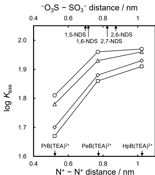
Fig. 7. Change in ion-association constant of anions associated with intra-atomic distance. NDS isomers: ○, 1,5-NDS; △, 1,6-NDS; □, 2,6-NDS; ◇, 2,7-NDS. Rearranged from a figure in Ref. 37.
