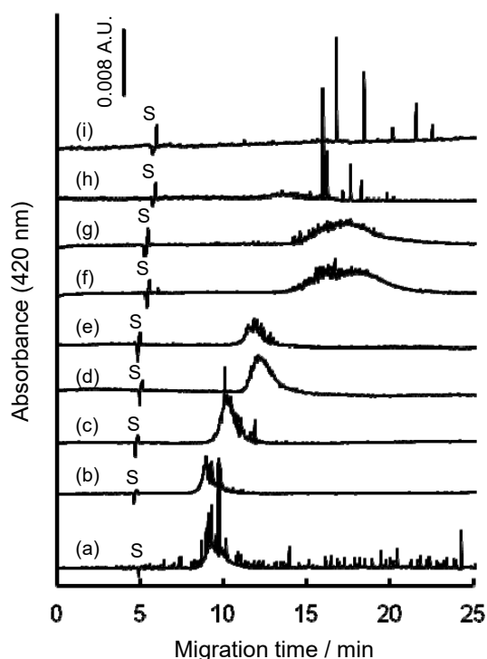
Fig. 11. Electropherograms of Graphene Nanoplatelets with varying concentrations of SDBS. Concentrations of SDBS (mmol dm -3 ): (a) 6; (b) 7; (c) 15; (d) 20; (e) 25; (f) 35; (g) 40; (h) 45; (i) 50. Concentration of graphene, 2 mg/mL; S, electroosmotic flow. Cited from Ref. 49.
