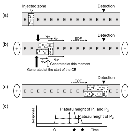
Fig. 16. Schematic migration diagram of two-substrates competitive reaction in CE/DFA. (a) – (c) Two products of P_1 and P_2 are formed from two substrates of S_1 and S_2 during the electrophoresis. An electropherogram (d) is expected by the competitive reaction; two products of P_1 and P_2 are detected as two-steps plateau signals by the enzymatic reaction. Cited from Ref. 72.
