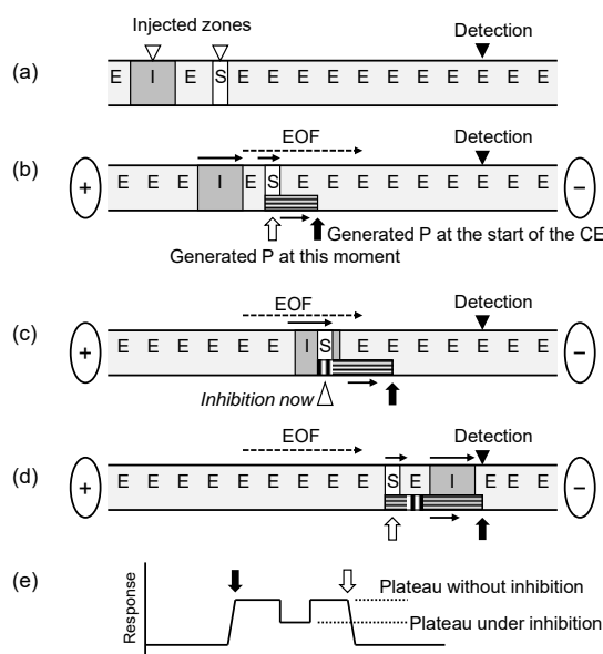
Fig. 15. Schematic diagram of the inhibition in CE/DFA by the tandem injections of a substrate and an inhibitor solutions (a) – (d), and a typical electropherogram (e). The inhibition occurs when the zones of a substrate (S) and an inhibitor (I) overlap by the electrophoretic migration. E: an enzyme contained in the separation buffer. Cited from Ref. 70.
