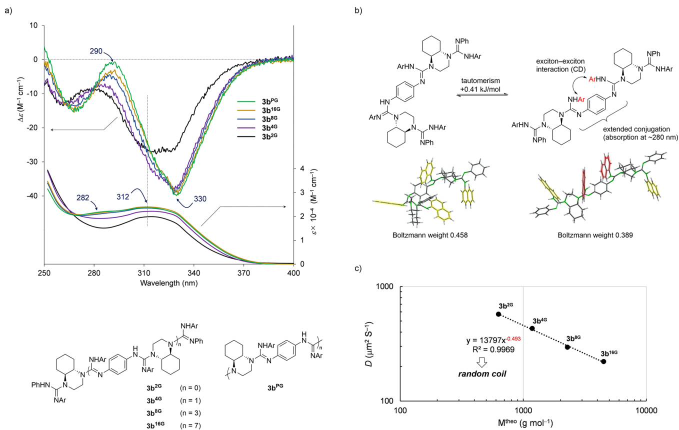
Figure 5. Optical and conformational aspects of 3b PG and its analogues (Ar = 1-naphthyl): (a) CD (25 °C) and absorption (ca. 25 °C) spectra of 3b 2G , 3b 4G , 3b 8G , 3b 16G , and 3b PG in CHCl 3 (0.02 M), (b) tautomeric and conformational preference of 3b 4G estimated by molecular mechanics calculations, (c) correlation between molar mass ( M^{\text{theo}} ) and self-diffusion coefficient ( D ) determined by DOSY.
