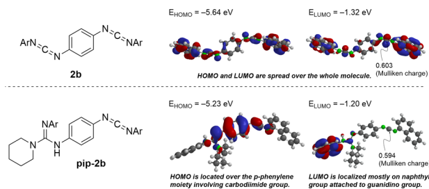
Figure 3. Frontier molecular orbitals and electronic properties of 2b and pip-2b estimated by DFT calculations (Ar = 1-naphthyl).
