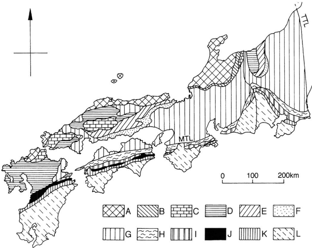
FIG. 1. — Zonal distribution of pre-Neogene orogenic units and accretionary complexes in SW Japan. A , Hida; B , Marginal Hida; C , Akiyoshi; D , Sangun; E , Maizuru; F , Ultra-Tamba; G , Mino-Tamba belts of the Inner Zone; H , Sambagawa-Mikabu; I , North Chichibu; J , Kurosegawa; K , South Chichibu belts; L , Shimanto Superbelts of the Outer Zone. MTL , Median Tectonic Line; TTL , Tanakura Tectonic Line.
