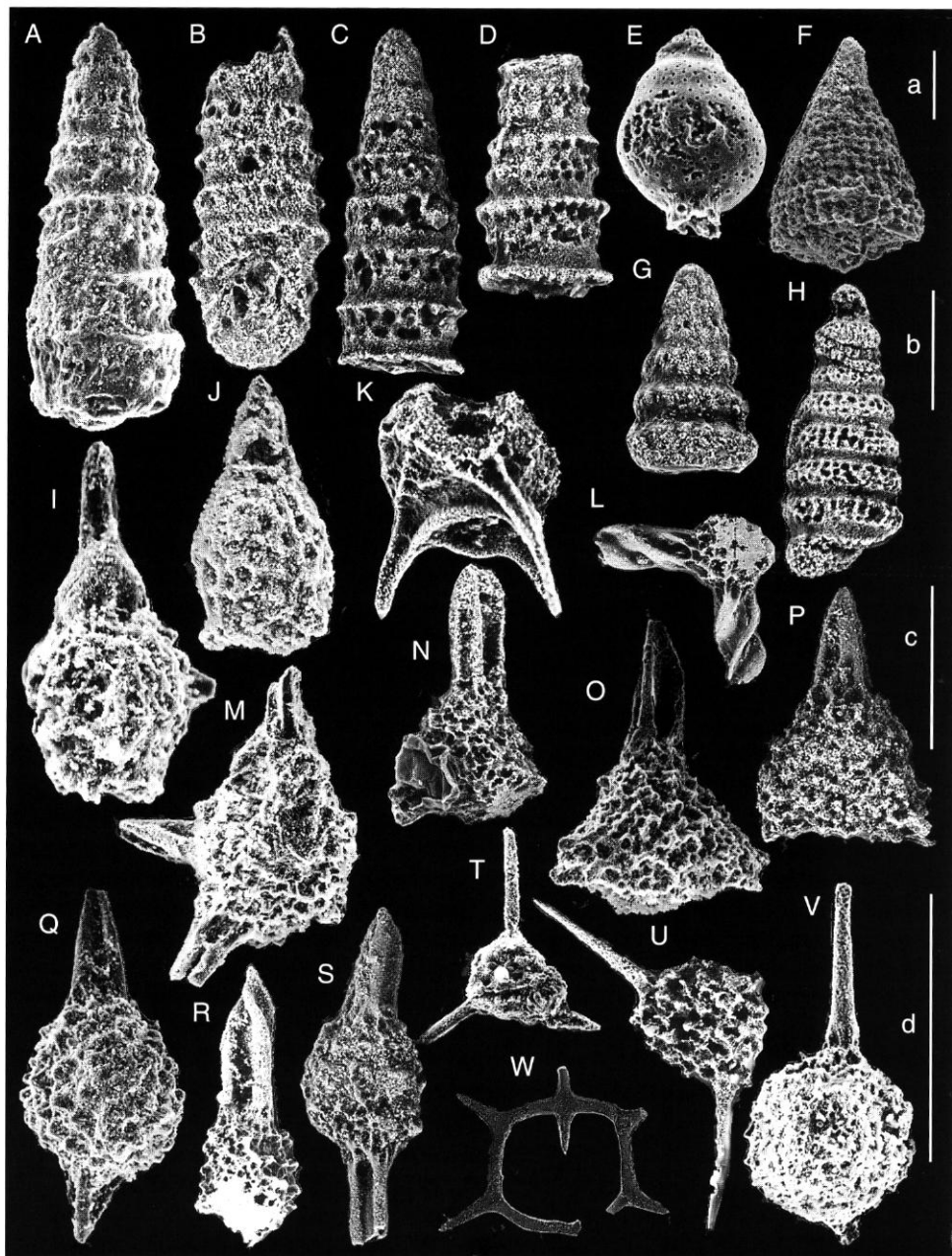
FIG. 5. — Middle-Late Triassic and earliest Jurassic radiolarians from the chert pebbles of the Ryoseki-Monobegawa group in East Shikoku. A , Triassocampe longicephalis Kozur & Mostler; B , Annulotriassocampe campanilis Kozur & Mostler; C , D , Triassocampe aff. scalaris Dumitrica, Kozur & Mostler; E , Gigi fustis De Wever; F , Parahsuum simplum Yao; G , Corum speciosum Blome; H , Pararuesticyrtium mediofassicum Kozur & Mostler; I , Hindedorcus holdsworthi Sugiyama; J , Theocorys sp. A of Nakaseko & Nishimura; K , Hozmadia reticulata Dumitrica, Kozur & Mostler; L , Tiborella cochleata (Nakaseko & Nishimura); M , Beturiella robusta Dumitrica, Kozur & Mostler; N , Eptingium manfredi robustum Kozur & Mostler; O , Eptingium nakasekoi Kozur & Mostler; P , Eptingium cf. manfredi Dumitrica; Q , Pseudostylosphaera spinulosum (Nakaseko & Nishimura); R , Pseudostylosphaera sp. C of Kojima & Mizutani, 1987; S , Pseudostylosphaera japonica (Nakaseko & Nishimura); T , Capnodocce sarisa De Wever; U , Trilonche japonica Nakaseko & Nishimura; V , Sarla (?) externa Blome; W , Acanthocircus vigrassi Blome. Scale bars: 100 \mu m; a, W; b, H, L-P, R-V; c, A-G, J, K, Q; d, I.
