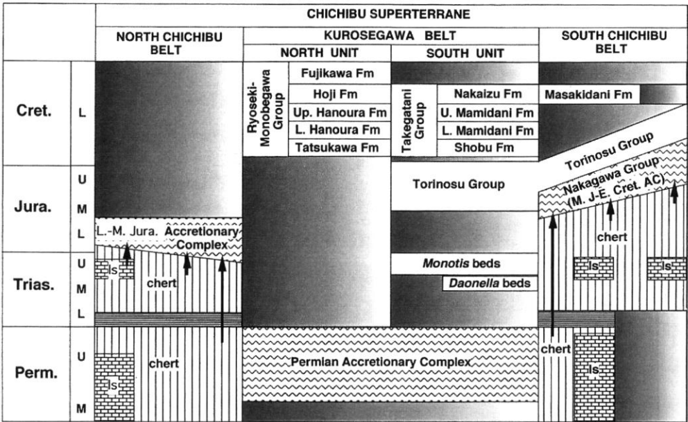
FIG. 11. — Stratigraphy of the upper Paleozoic and Mesozoic formations in the North Chichibu, South Chichibu and Kurosegawa belts in the Chichibu Superterrane, East Shikoku.
