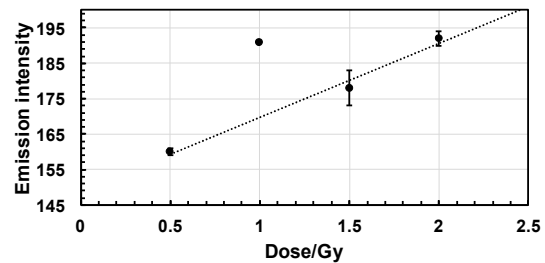
Figure 6. Relationship between emission intensity measured by a portable fluorometer (FC-1) and dose. 80 kV X-rays were irradiated to the CR-39 sticks doped with MV @ silica NCs.
