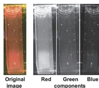
Figure 2. Emission and decomposed images of CR-39 stick doped with MV @ silica NCs irradiated by 10 Gy of 6 MeV X-rays.
